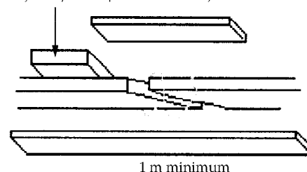
Brace which does not allow the normal positioning of the fish plate Jaube de force empêchant la position normale de la joue
